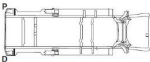
UNDERBODY VIEW
